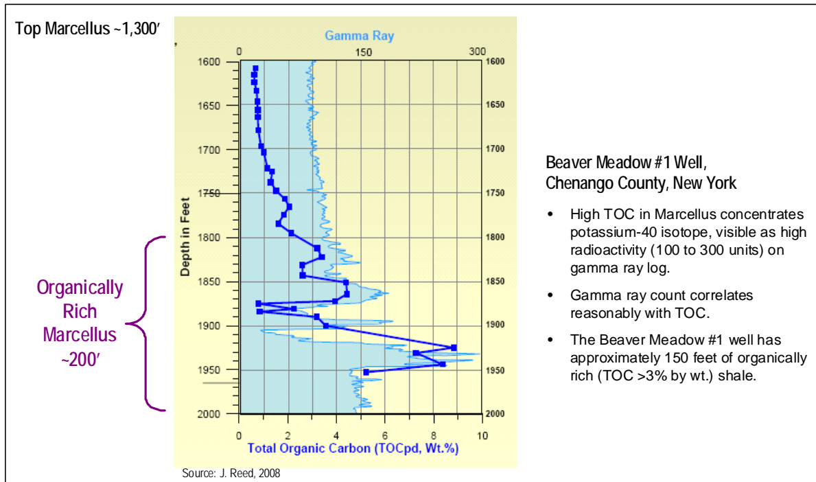
Figure 5. Relationship of Gamma Ray and Total Organic Carbon
